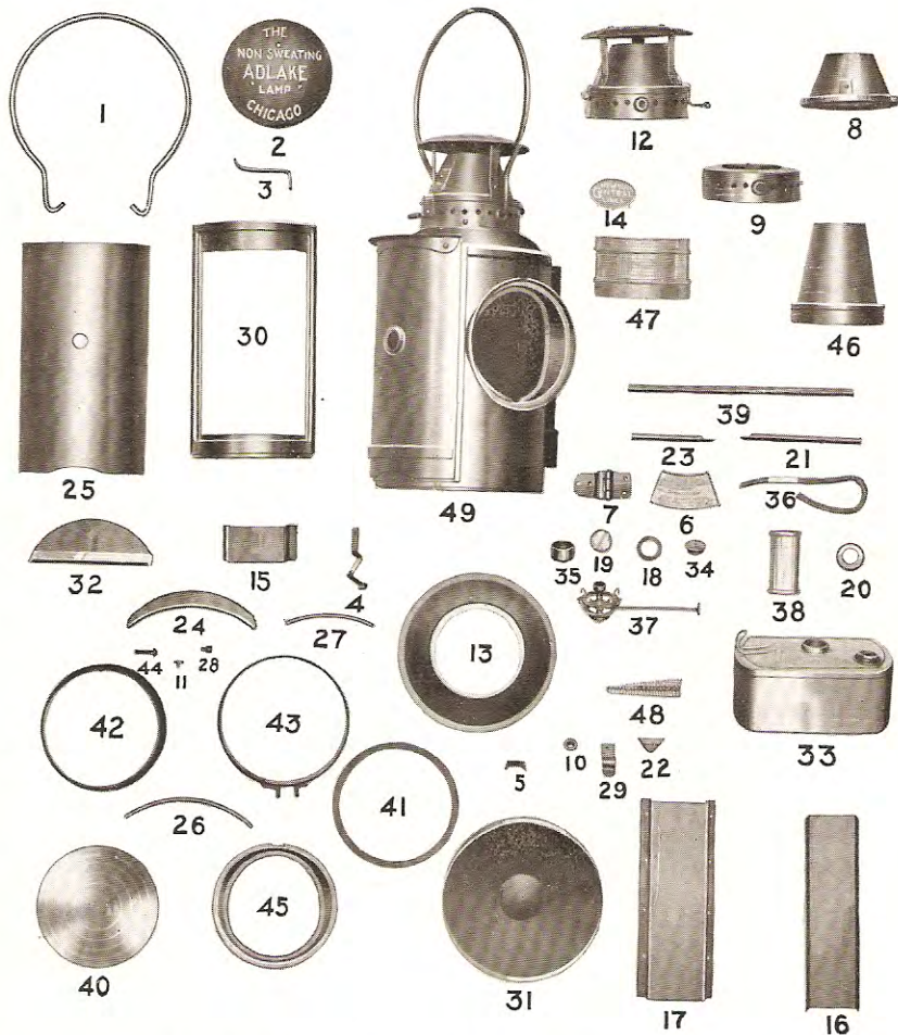
Parts of N. Y. C. Standard Semaphore Lamps
